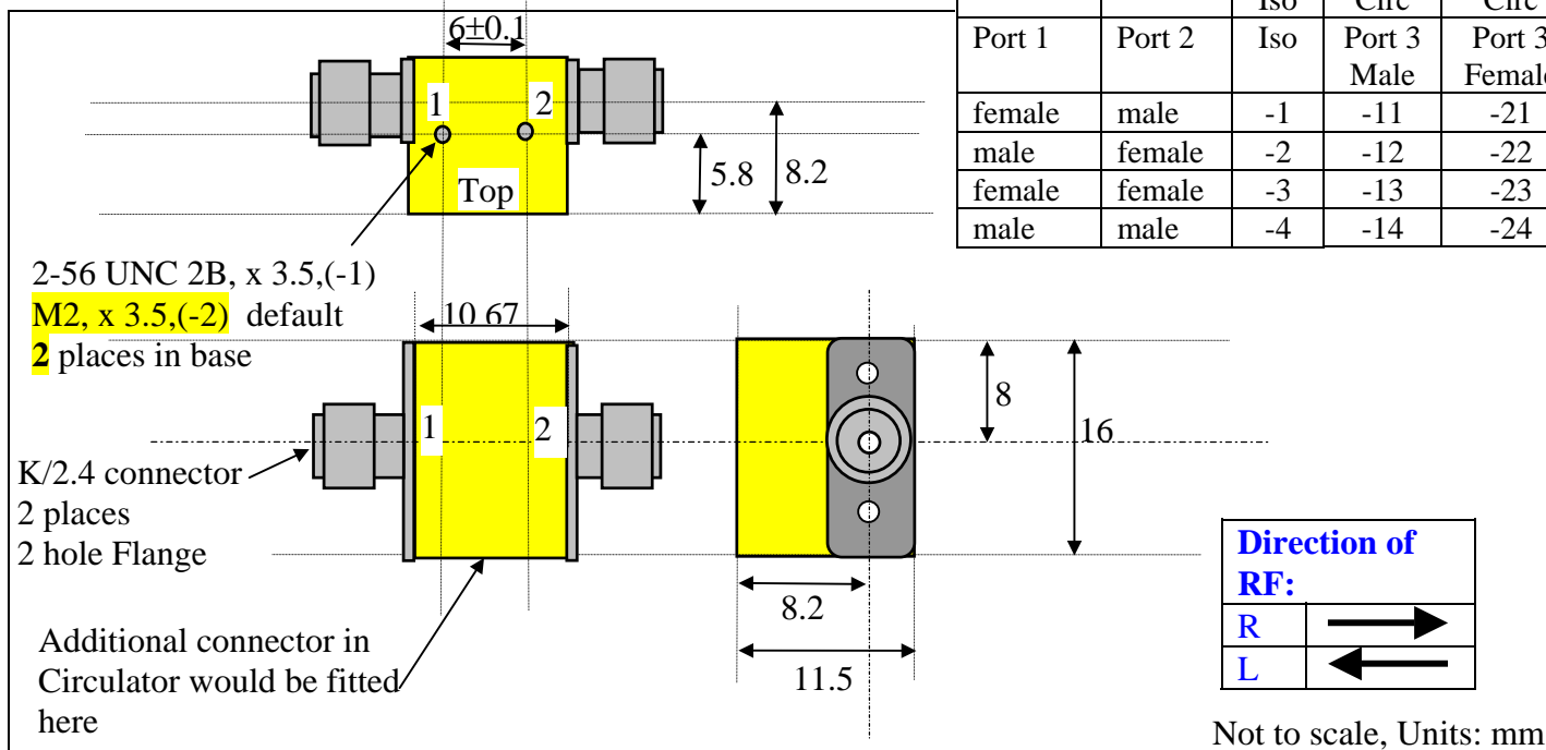
K/2.4 Connector options
